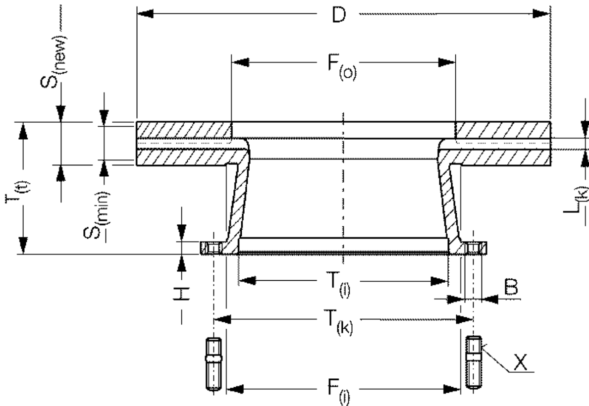
DOUBLE FLANGE TYPE
