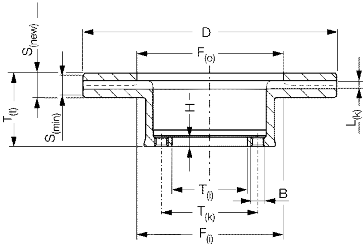
CONICAL TYPE
